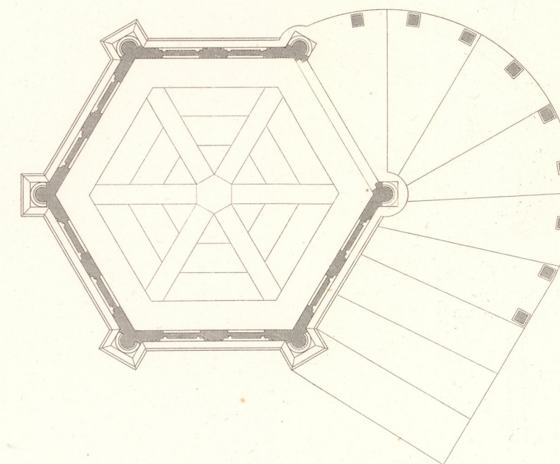
Plan
