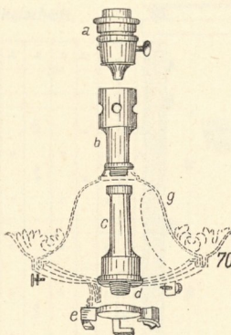
51. Invertbrenner.
