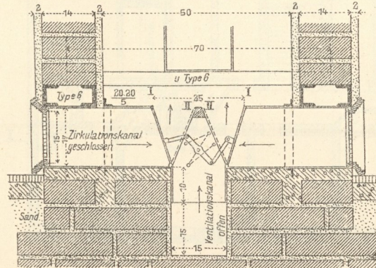
c. Detailschnitt I. II.
