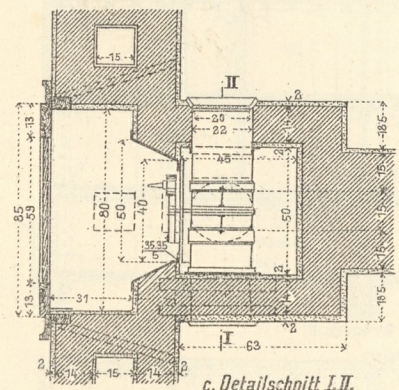
c. Detailschnitt I. II.
