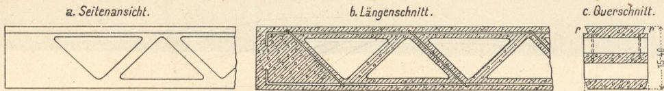
2. Eisenbetondecke, System Visintini.
