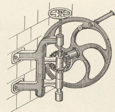
31. Wand-Bohrmaschine.
