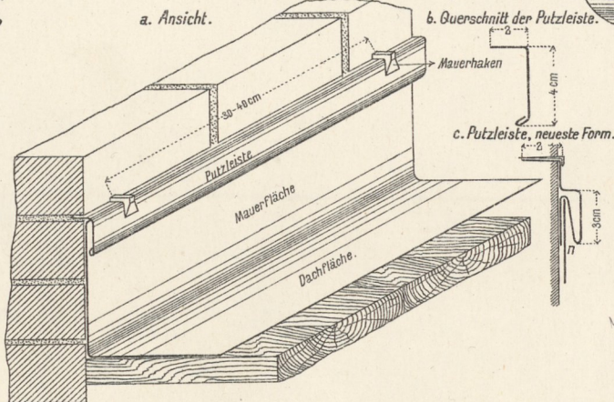
9. Maueranschlüsse (Wandixen).
