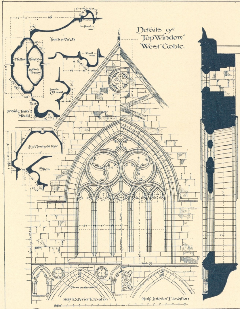
Fig. 284—286. Klosterkirche zu Saint Mirren Paisley. (The Building News 1888.)
