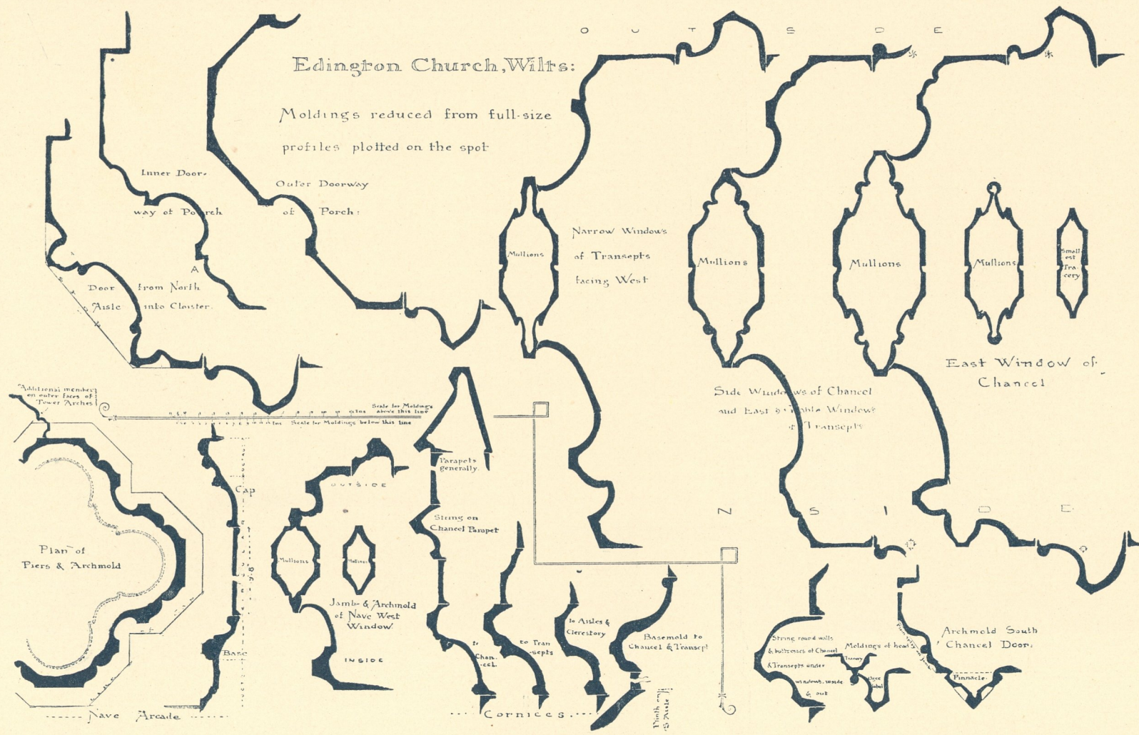
Fig. 290/291. A. d. Kirche zu Edington (Wiltshire). The Building News.
