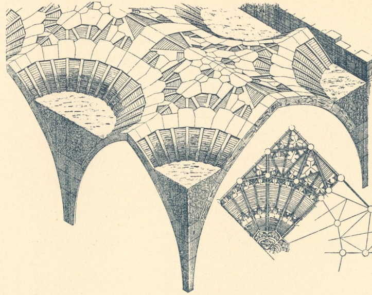
Fig. 296. A. d. Marienkirche zu Sherborne. (The Building News 1883.)
