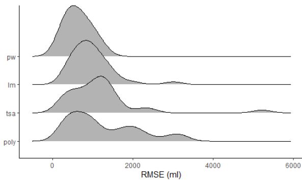
Figure 3: Whole sample extrapolation error of the cumulative fluid intake (48h of modelling, 24h of prediction). Piecewise linear modelling (pw), linear modeling (lm), time series analysis (tsa), polynomial terms (poly), root mean squared error (RMSE).
