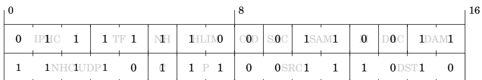
Figure 2.26: Link-Local IPv6 an UDP header to IPHC example
