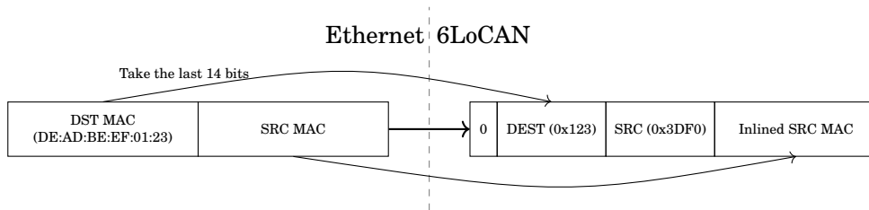
Figure 3.10: Ethernet to 6LoCAN Address Translation
