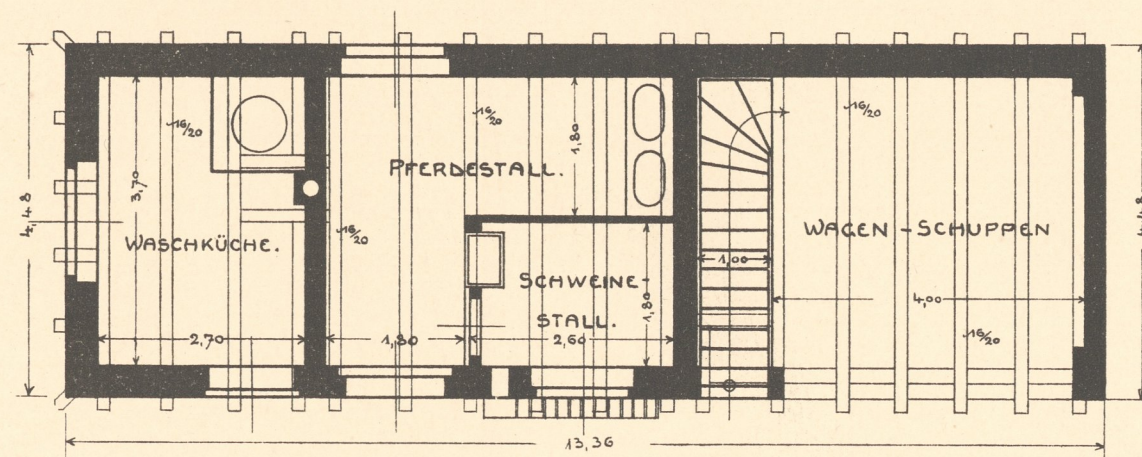
ERDGESCHOSS.
