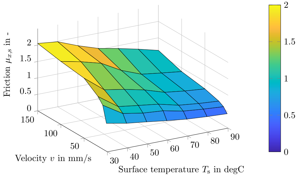
Figure 3.14.: Longitudinal coefficient of friction \mu_{x,s} over surface temperature T_s and velocity v on a rough aluminium surface with section temperature T_p = 50 degC and section load m_p = 9.12 kg
