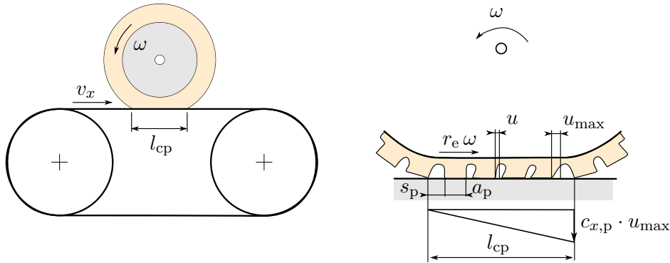
Figure 4.3.: Tyre tread section investigation concept; left, assumed tyre velocities on a flat track test rig; right, simplified shear stress distribution depending on the tyre contact length position, adapted from [Rill, 2015]
