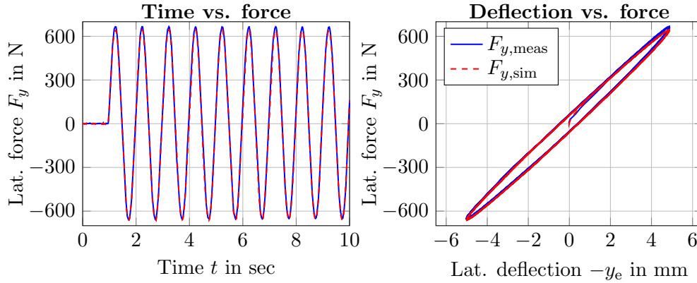
Figure 6.3.: Validation of the parameterised Voigt-Kelvin model with measurements of a deflection sine manoeuvre for the non-rolling tyre with tyre load F_z = 3600 N, deflection amplitude of A_{\text{sine}} = 5 mm and a frequency of f_{\text{sine}} = 1 Hz, adapted from [Hackl et al., 2016a]
