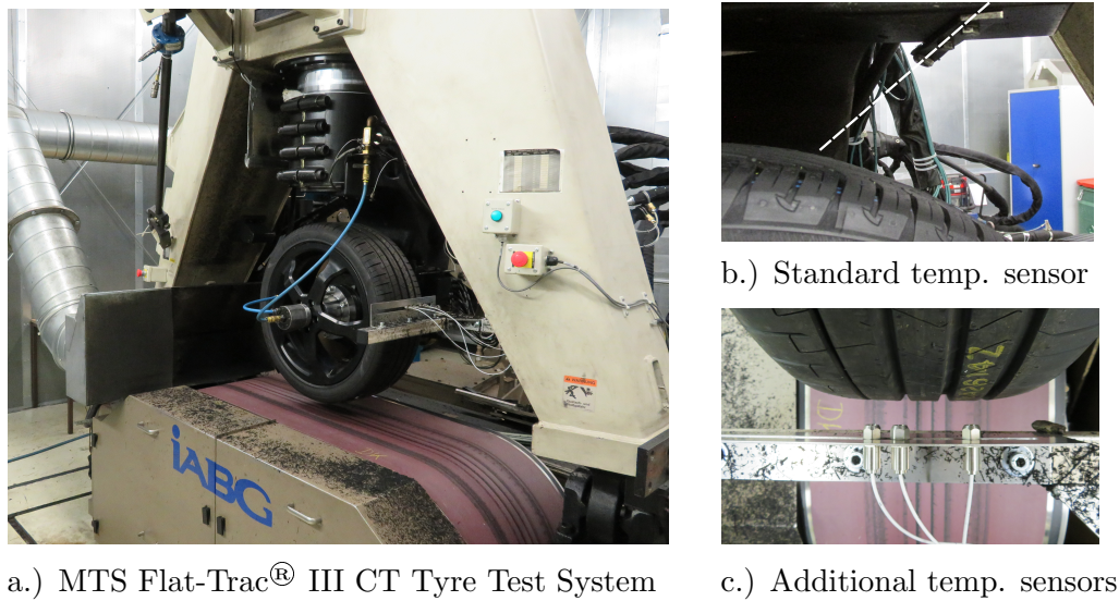
Figure 4.2.: Illustrations of the used MTS Flat-Trac ® III CT (Cornering & Traction) Tyre Test System used; a.) overall test bench representation, b.) mounting position of the standard temperature sensor, c.) positioning of the three additional temperature sensors
