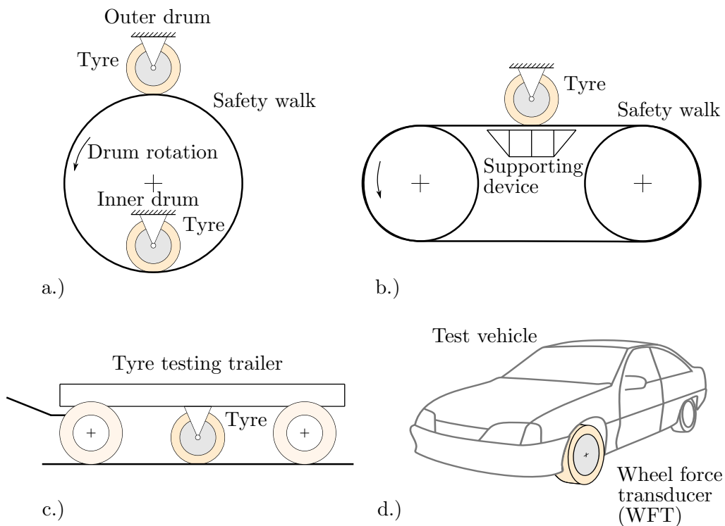
Figure 4.1.: Schematic representation of common tyre test bench systems adapted from [Rill, 2012]; upper left, inner and outer drum applications; upper right, flat track tyre test bench; bottom left, tyre trailer system; bottom right, schematic representation of tyre measurements under real driving operation
