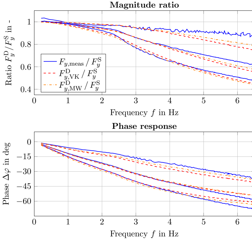
Figure 6.15.: Magnitude ratio and phase response in lateral direction for the PP0 tyre based on the frequency sine sweep for three different wheel loads F_{z,\text{PP0}} ; the simulated steady-state force serves as basis for the measured F_{y,\text{meas}} in solid blue, the simulated Voigt-Kelvin F_{y,\text{VK}}^D in dashed red and the simulated Maxwell F_{y,\text{MW}}^D force in dot-dashed orange
