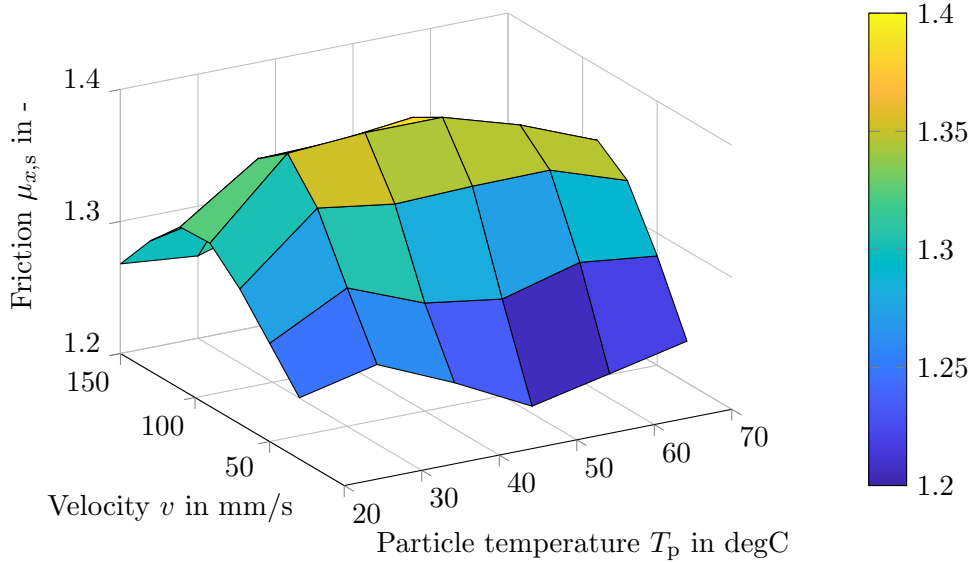
Figure 3.13.: Longitudinal coefficient of friction \mu_{x,s} over section temperature T_p and velocity v on P120 sandpaper surface with track temperature T_s = 30 degC and section load m_p = 12.58 kg
