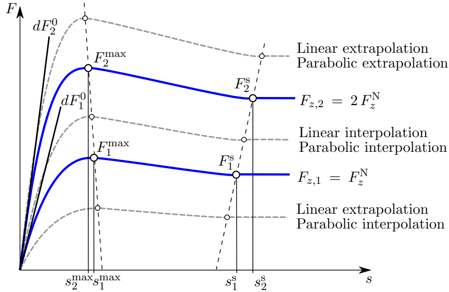
Figure 4.7.: Generic tyre model characteristics with five representative parameters, each at a defined payload F_{z,1} = F_z^N and doubled F_{z,2} = 2 F_z^N , adapted from [Rill, 2015]
