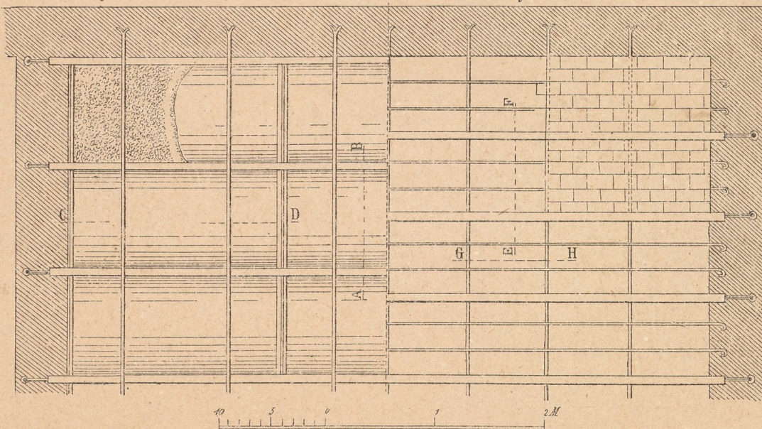
System XIII. Fig. 5.
