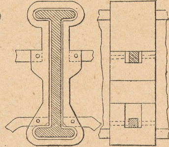
Detail X. Fig. 7.
