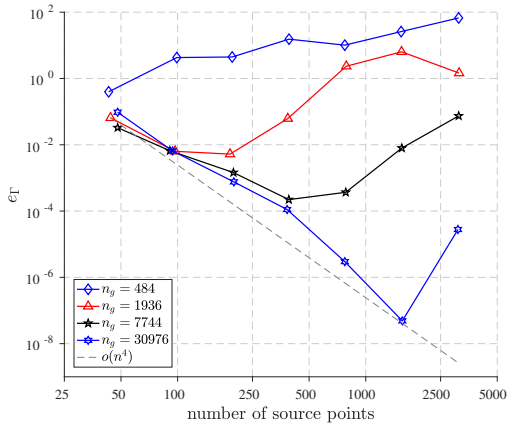
Figure 5.7: Error convergence for the parametric MFS verification example
