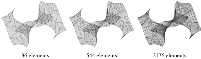
Figure 6.3: Three triangulations of the considered gyroid surface
