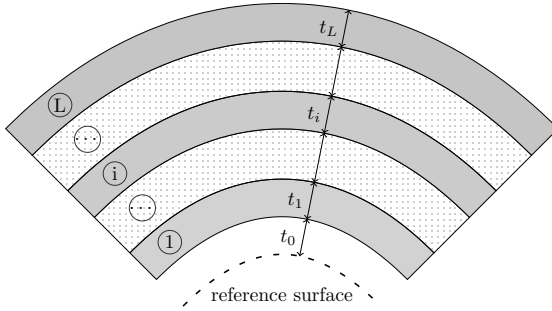
Figure 3.2: Layup of the shell
