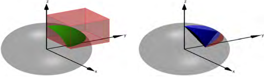
Figure 4.4: Limitations of the closest point projection lift
