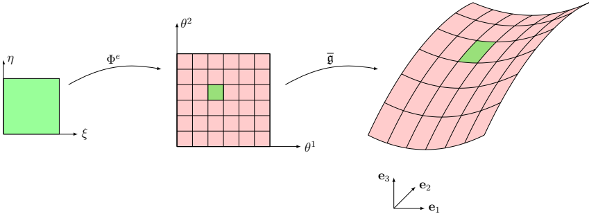
Figure 4.3: Geometry mappings for parametrically given shells
