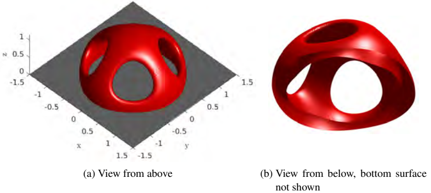
Figure 6.5: Geometry of the orthocircle problem
