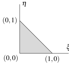
Figure 4.1: Reference triangle
