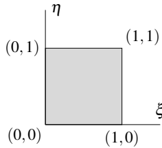
Figure 4.2: Reference quadrilateral
