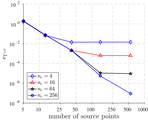
Figure 5.10: Error e_T for the exterior fluid in case of the coupled MFS-FEM: elastic structure and implicitly given reference surface
