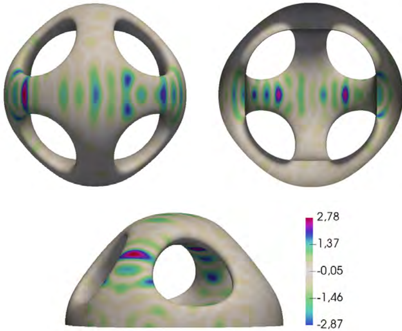
Figure 6.7: Real part of the pressure [\text{N}/\text{m}^2] at the boundary from different perspectives, n_s = 9579
