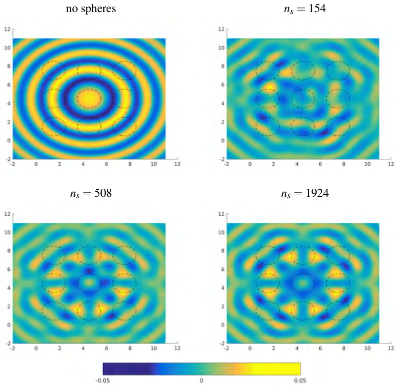
Figure 6.9: Real part of the pressure at the evaluation surface
