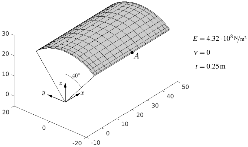
Figure 6.1: Problem description of the Scordelis-Lo-Roof
