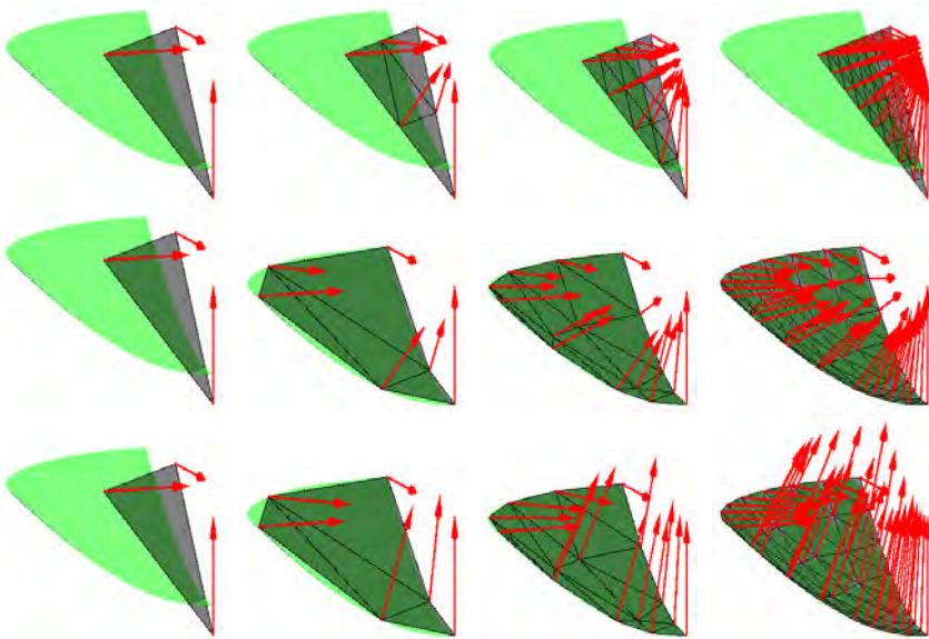
Figure 4.5: Refinement without (upper row) and with (lower row) lifting the vertices, the red arrows indicate the search directions
