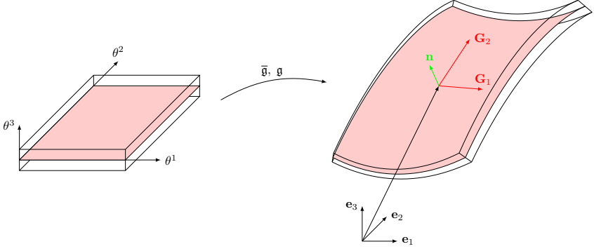
Figure 3.1: Parametrization of a shell
