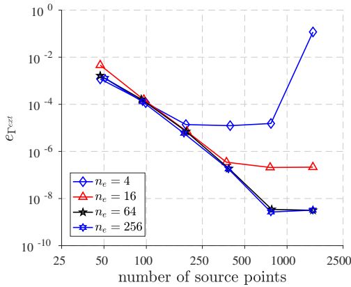
Figure 5.11: Error e_T for the exterior fluid in case of the coupled MFS-FEM: poroelastic structure and parametrically given reference surface
