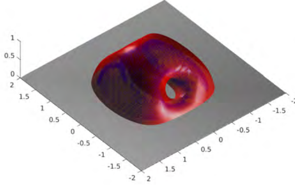
Figure 5.8: Configuration of the implicit MFS verification example: Sound hard plane at z = 0 (gray), sound hard surface \Gamma (red), MMS source point (black), MFS source points (blue)
