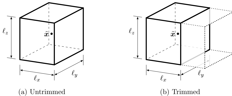
Figure 7.30: Discretization of a unit cube by (a) regular patches and (b) trimmed patches.
