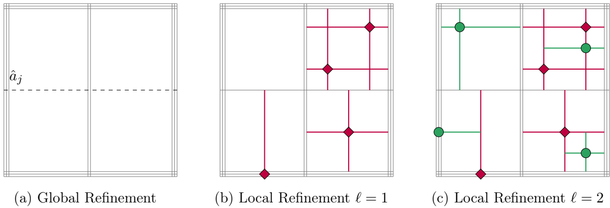
Figure 5.2: Subsequent refinement of integration elements defined by the tensor product of \Lambda_I = \{0, 0, 0, 1, 1, 2, 2, 2\} and \Lambda_J = \{0, 0, 0, 2, 2, 2\} . (a) Global refinement by inserting \hat{a}_j = 1 into \Lambda_J . (b) Subdivision into local elements by refinement points of the first refinement level which are denoted by diamonds. (c) Further local refinement by a higher refinement level indicated by circles.
