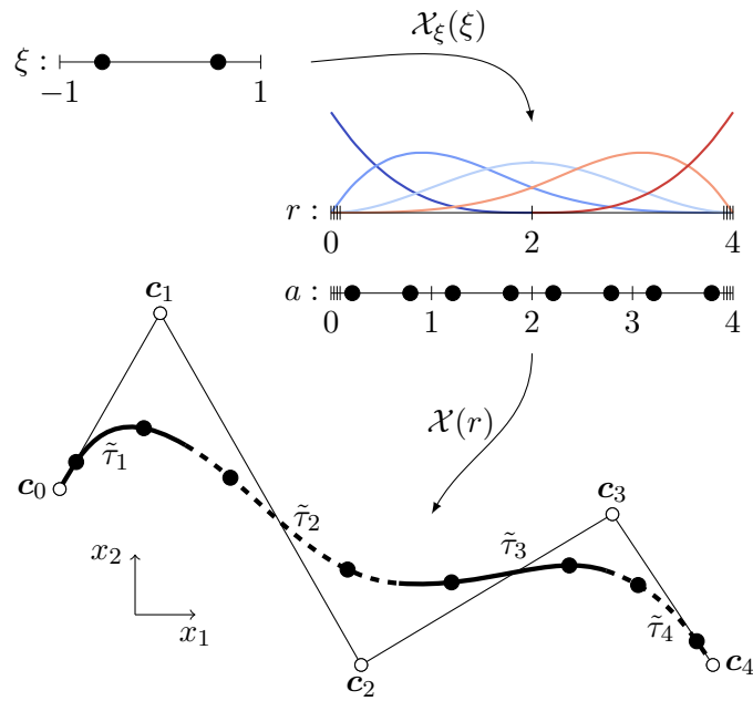
Figure 5.1: The geometry of a cubic B-spline curve is defined by control points \mathbf{c}_i and the knot vector \Xi = \{0, 0, 0, 0, 2, 4, 4, 4, 4\} . The elements \tilde{\tau}_j along the curve are defined by \Lambda = \{0, 0, 0, 0, 1, 2, 3, 4, 4, 4, 4\} in the parameter space. Each element is equipped with a two point quadrature rule defined in the reference interval \xi \in [-1, 1] .
