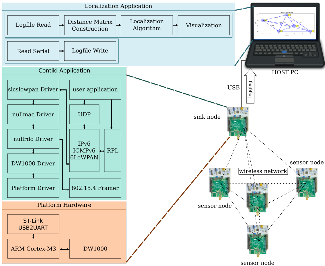
Figure 3.4: Block diagram of NetLoc's architecture.
