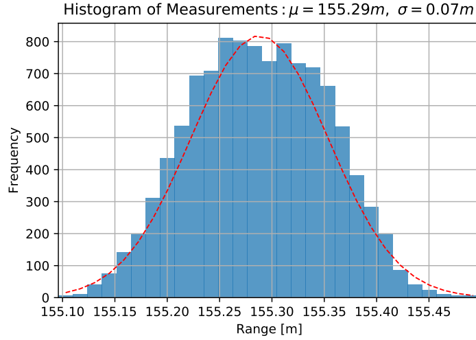
Figure 4.7: Histogram of TWR measurements.
