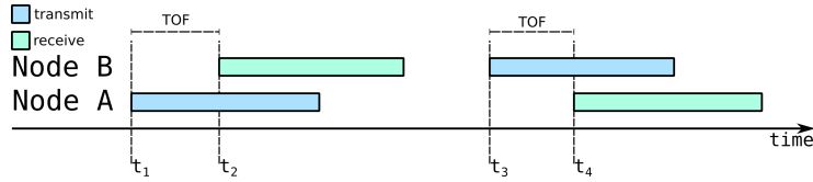
Figure 2.8: Single-Sided Two-Way Ranging.
