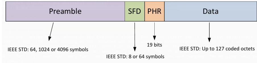
Figure 2.5: UWB PHY frame structure supported by the DW1000 [26, Figure 31].
