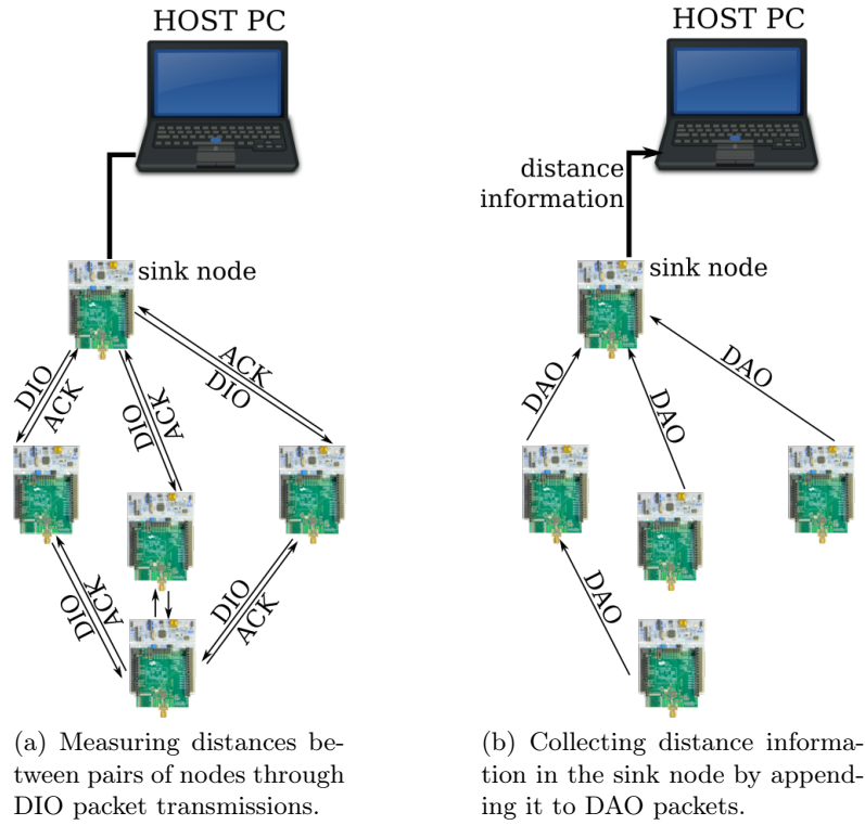
Figure 3.1: Packet exchange to measure the TOF of DIO packets (a) and then collect the distance information in the network's sink by appending it to DAO packets (b).
