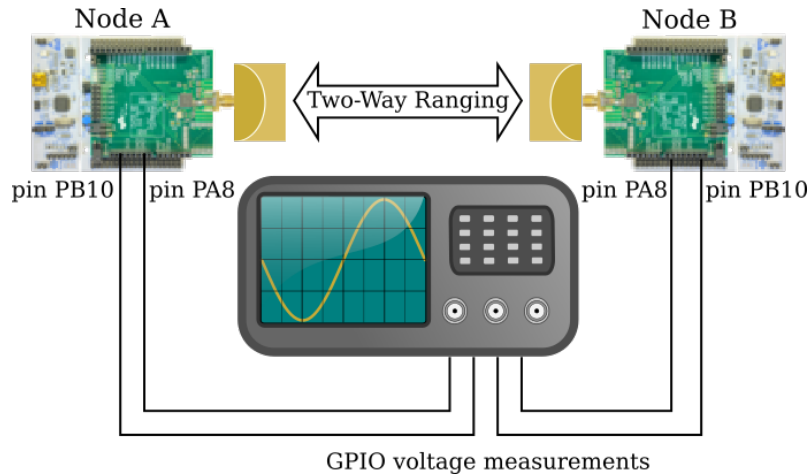
Figure 5.3: Test setup to measure processing times and communication times during DS-TWR using an oscilloscope.
