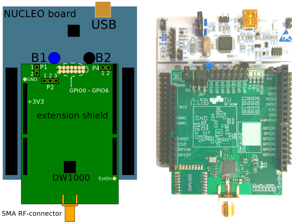
(a) Block diagram of the UWB extension shield stacked on top of the NUCLEO-L152RE board.
