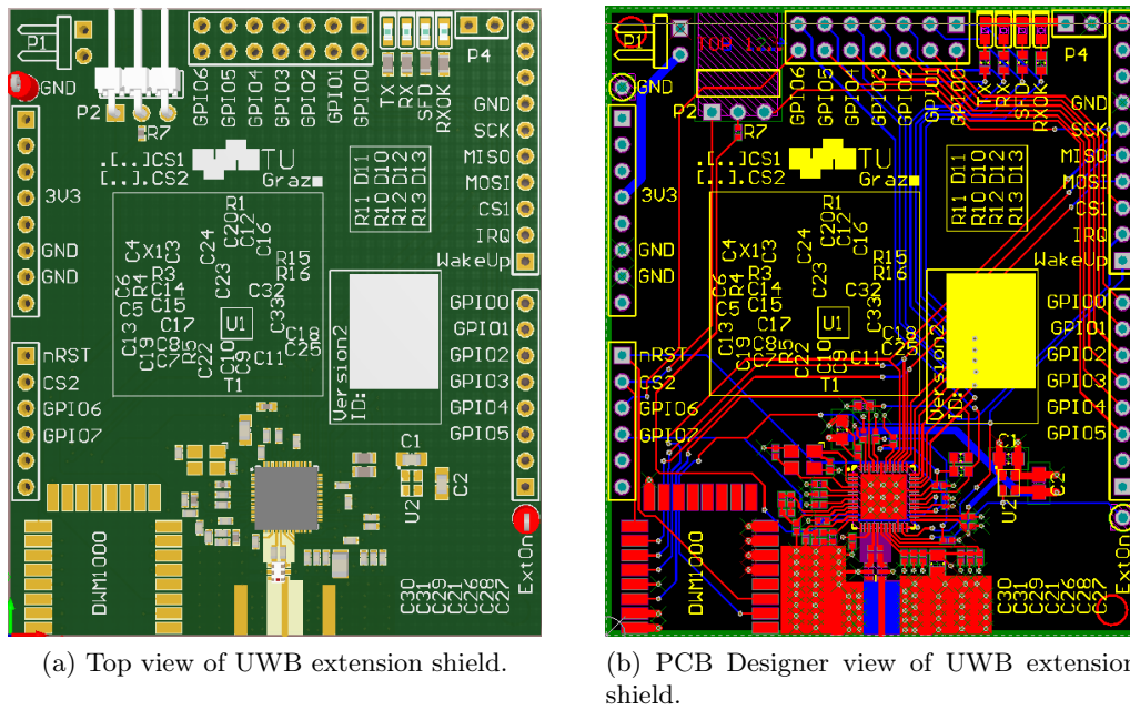
Figure 4.2: UWB extension shield design.
