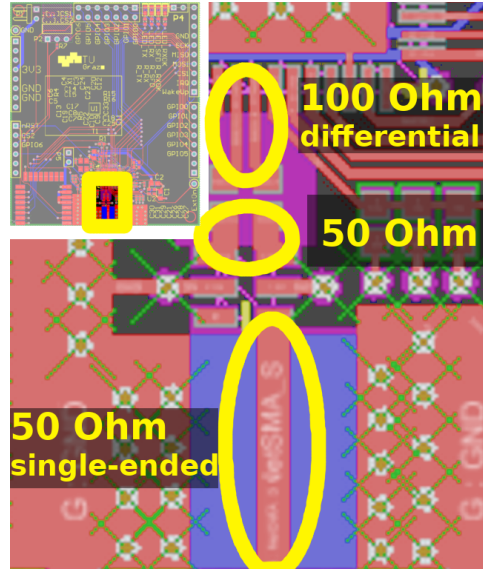
Figure 4.4: RF transmission lines.
