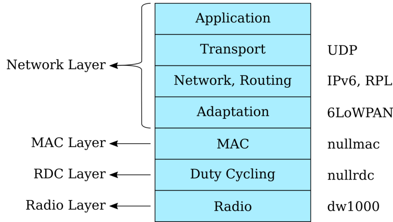
Figure 2.1: Contiki's network protocol stack [4].
