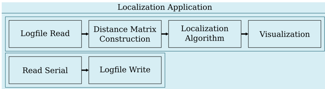
Figure 5.5: Building blocks of NetLoc’s localization application.
