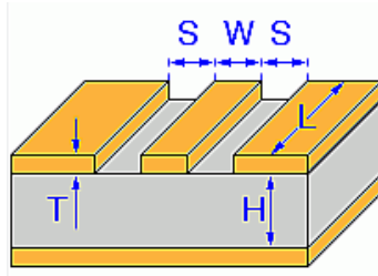
Figure 4.5: Scheme for transmission lines with co-planar wave guide and ground plane.
