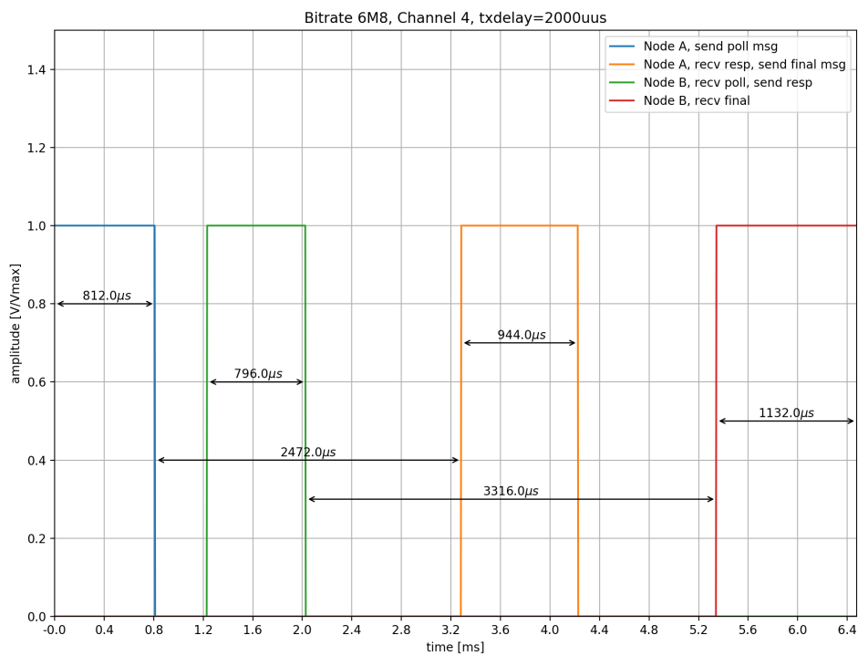
Figure 5.4: Measured time intervals during a DS-TWR measurement between two nodes.
