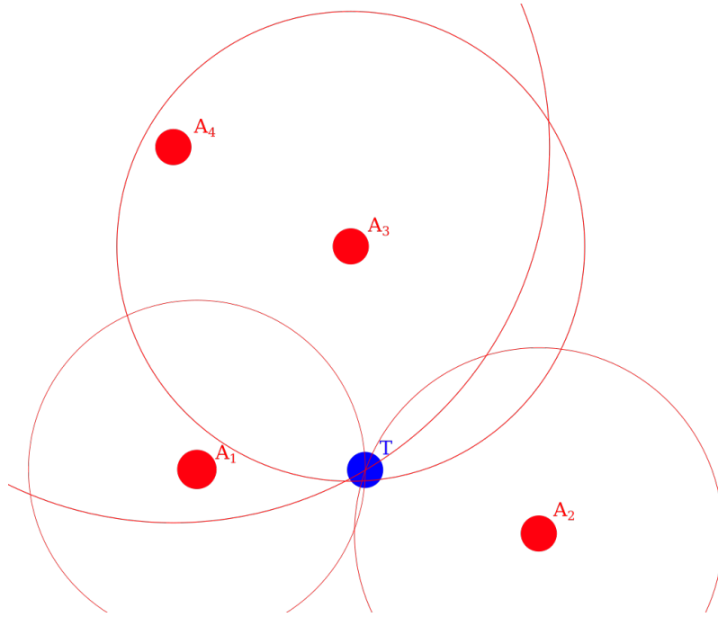
Figure 2.10: Two-dimensional positioning based on four distance measurements. The red dots and circles represent anchors ( A_1 - A_4 ) and their distance measurements, respectively. The blue dot is the calculated position of the tag ( T ), where all circles intersect.
