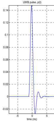
Figure 2.4: UWB pulse shape according to IEEE 802.15.4(a) [47, Figure 16-13].
