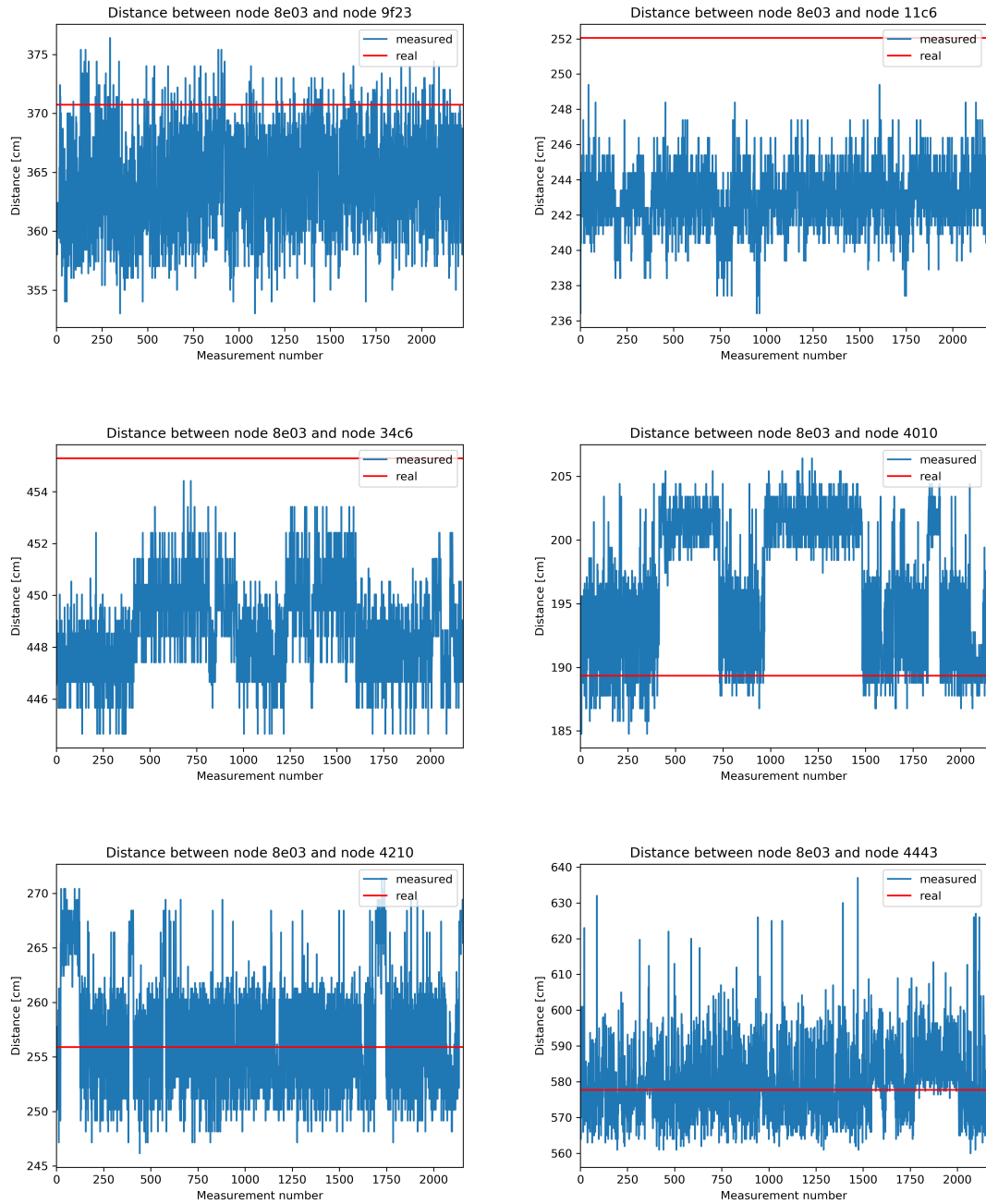
Figure 6.2: Distance measurements of node 8e03 to its neighbors 9f23, 11c6, 34c6, 4010, 4210, and 4443.
