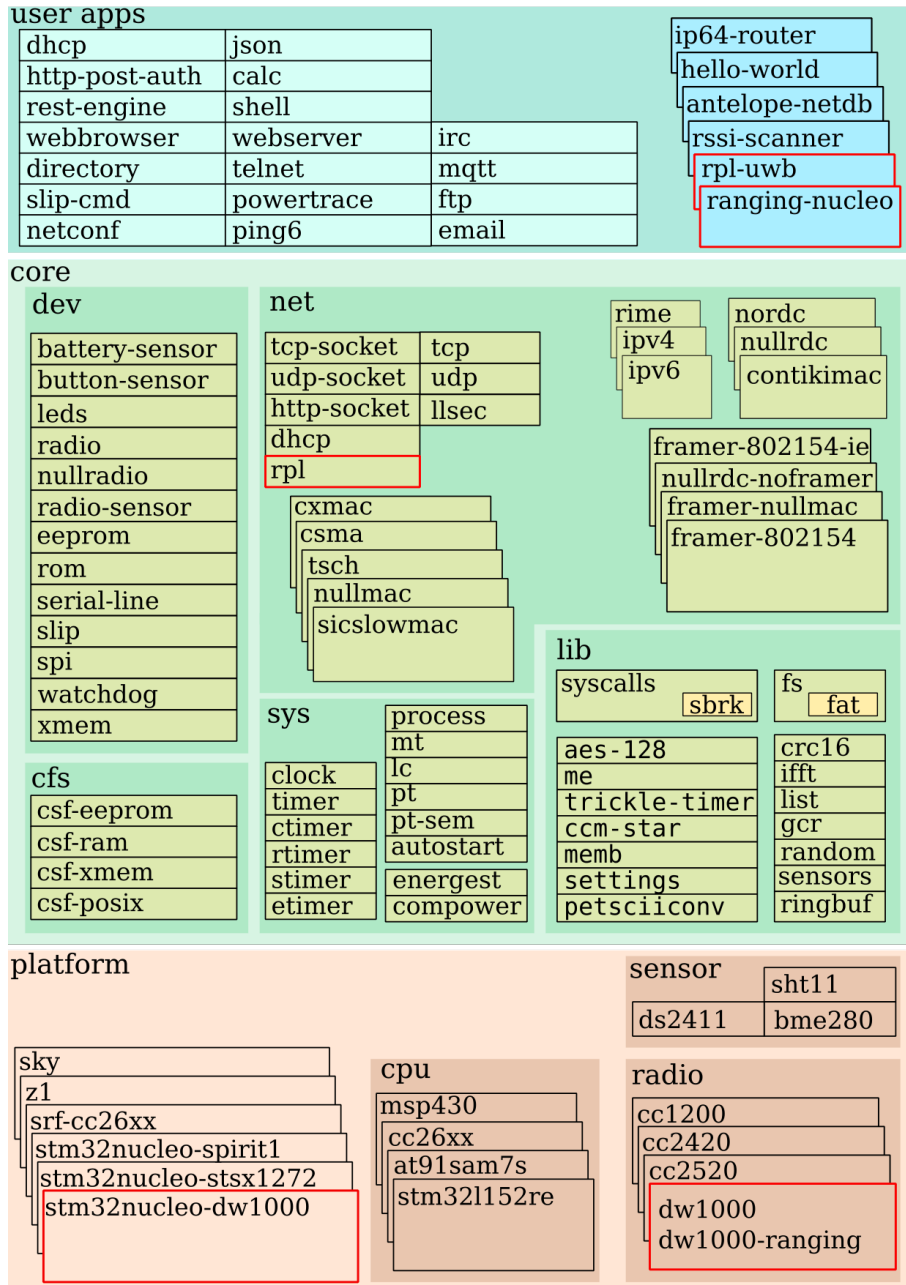
Figure 2.2: A block diagram of Contiki’s software architecture. Blocks that are of special interest for the NetLoc system have red borders. Overlapping blocks exclude each other. Non-overlapping blocks can exist concurrently. User applications ( rpl-uwb , hello-world , ...) and application layer protocols ( telnet , mqtt , ...) are on the top of the diagram in the user apps block. Contiki’s kernel, its coffee file system cfs , network- and MAC protocols, as well as timer and hardware abstractions are part of the core block. The platform block contains all hardware dependent modules; higher-level modules are hardware-independent.
