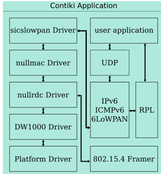
Figure 5.1: Building blocks of NetLoc's Contiki application
