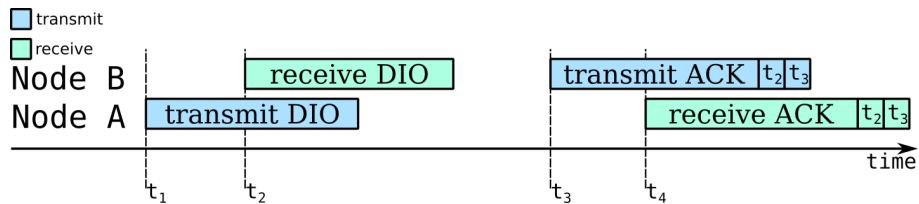
Figure 3.2: Principle of NetLoc to derive distance information. Node A sends a DIO packet to node B with an active ranging flag in the PHR of the packet. Node B recognizes this flag and appends the reception timestamp of the DIO packet ( t_2 ) and the transmission time of the ACK packet ( t_3 ) before sending the ACK.
