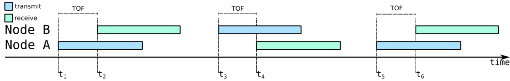
Figure 2.9: Double-Sided Two-Way Ranging.
