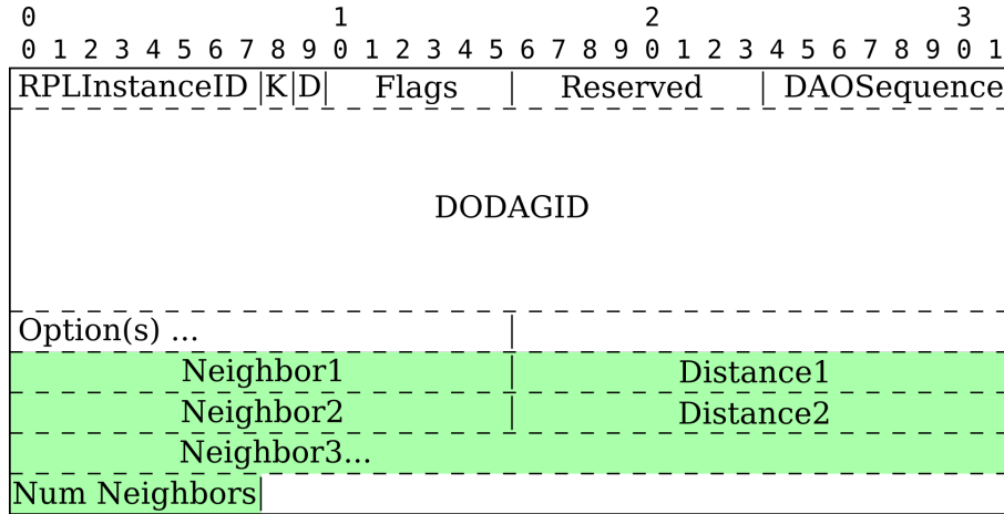
Figure 5.2: Format of the DAO Base Object [86, Section 6.4.1.]. Appended new fields are colored green.
