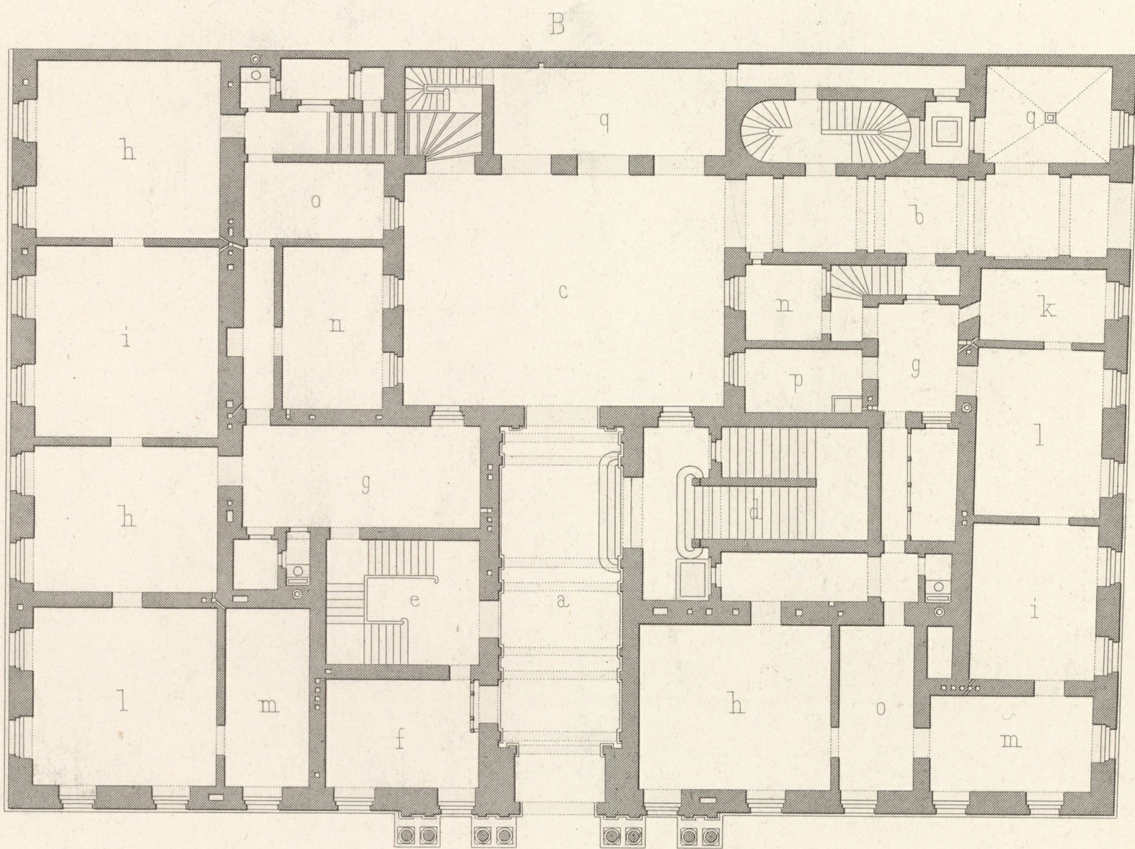
B. ERDGESCHOSS.
