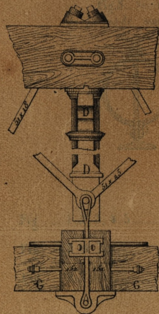
Fig 3. Montant intermediaire Elevation laterale
