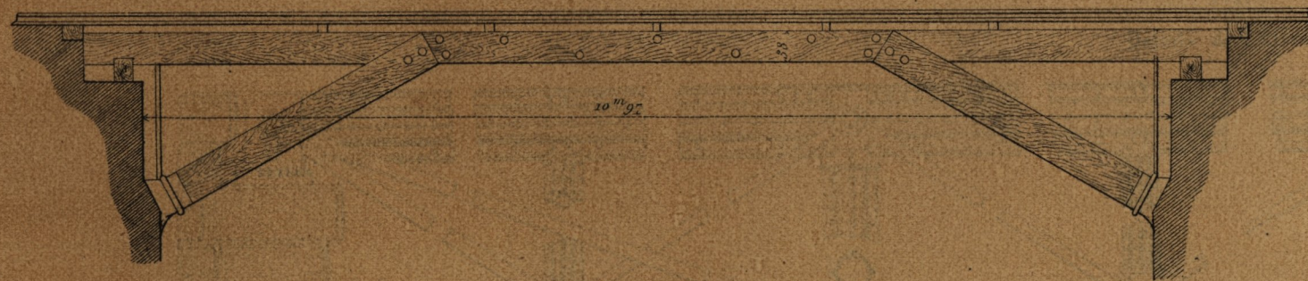
Fig 5. Elevation
