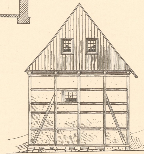
Abb. 7. Speicher.
