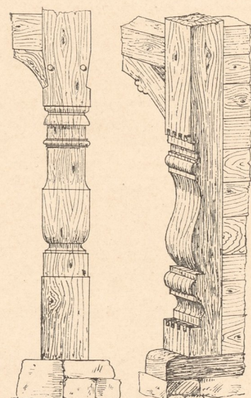
Abb. 9. Pfostendetails.
