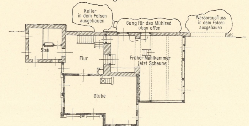
Erdgeschoss.
