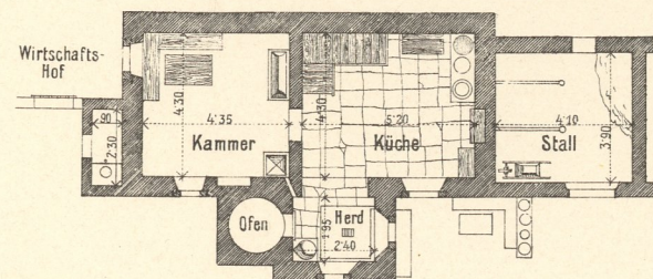
Erdgeschoss.
