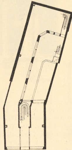
Erdgefchofs.
