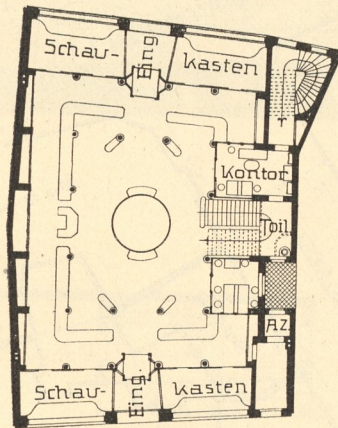
Erdgeschoss.
