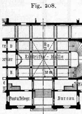
Vom Hôtel Beauvillage in Ouchy. \frac{1}{500} n. Gr.
