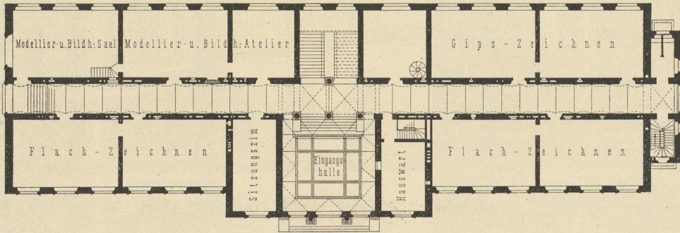
Erdgefchofs.
