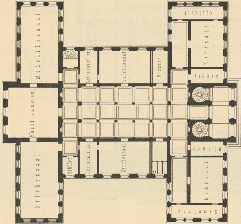
Erdgeschoss.
