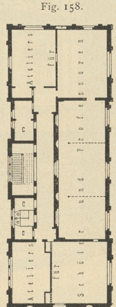
II. Obergeschoss.
