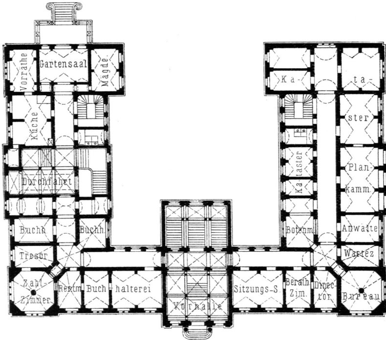
Erdgefchofs.
