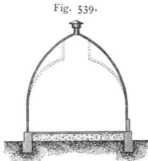
Tollet's Pavillon-Typus.
