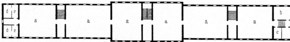
I., II. u. III. Obergechofs.
