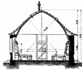
Tollet's Lager-Pavillon.
