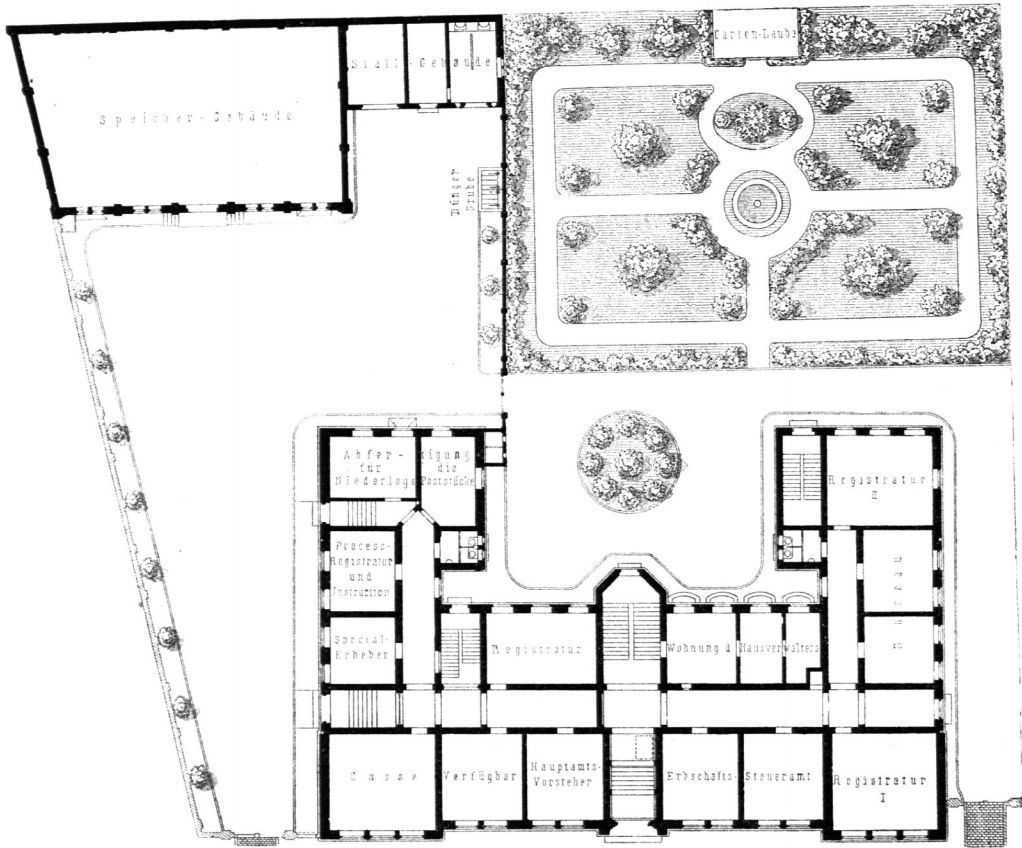
Erdgefchofs.
