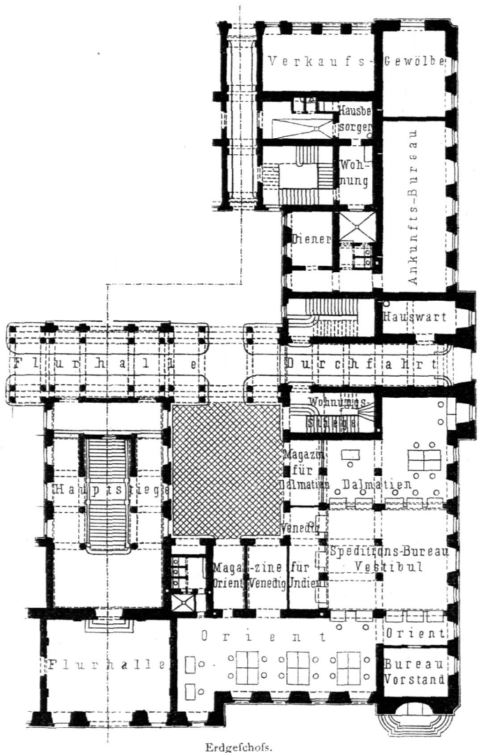
Erdgechofs.
