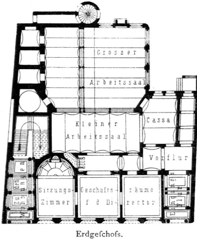
Erdgeschoss.
