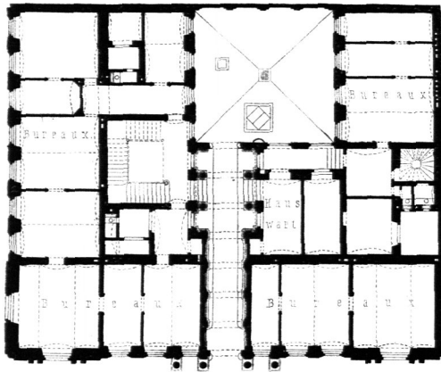
Erdgeſchoſs.
