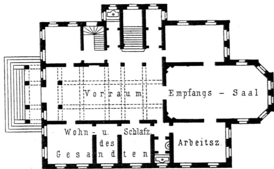
Erdgechofs.
