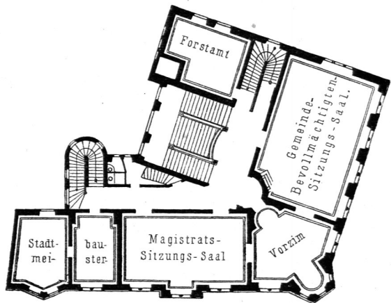
II. Obergeschofs.
