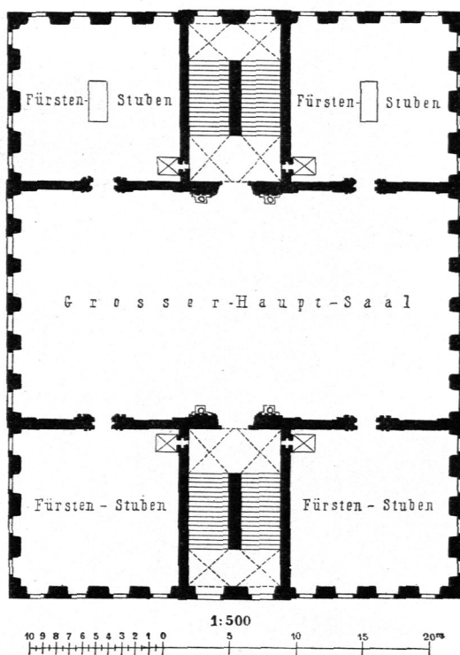
Rathhaus zu Augsburg. — II. Obergechofs.
