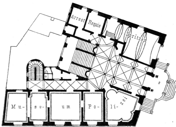
Erdgeschofs.
