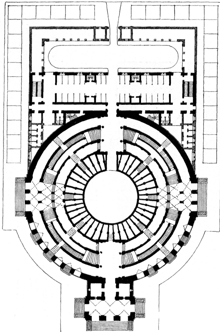
Erdgeschoss.
