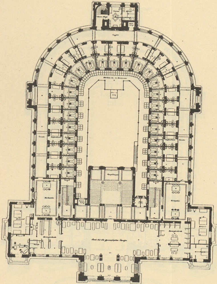
Kaiserbad zu Carlsbad. — I. Obergeschofs. — \frac{1}{500} n. Gr.
