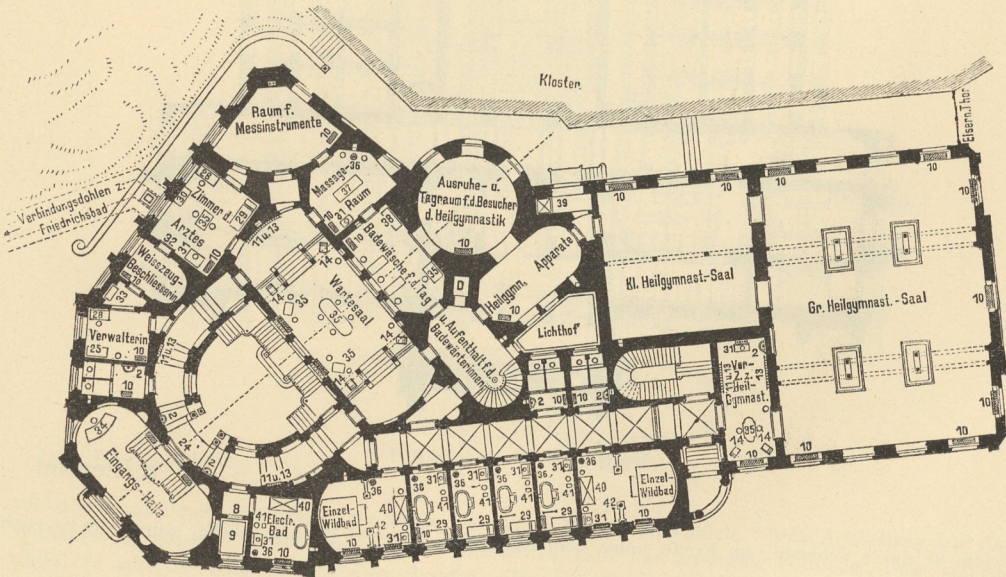
Erdgeschoss.
