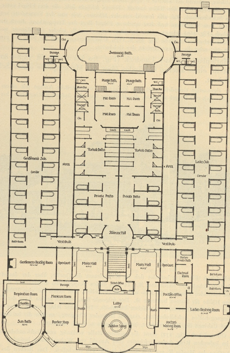
Erdgechofs.
