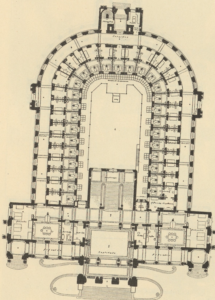
Erdgefchofs. — \frac{1}{550} n. Gr.
