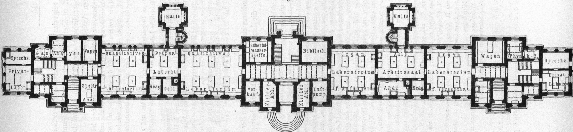
Erdgeschoss.
