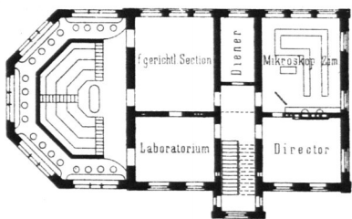
Erdgeschoss.
