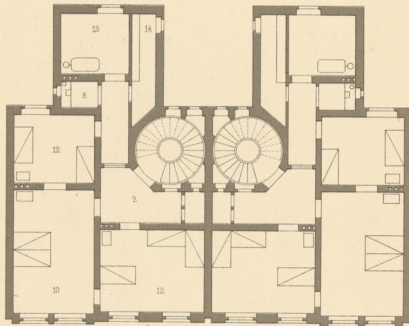
Ier Stock.
