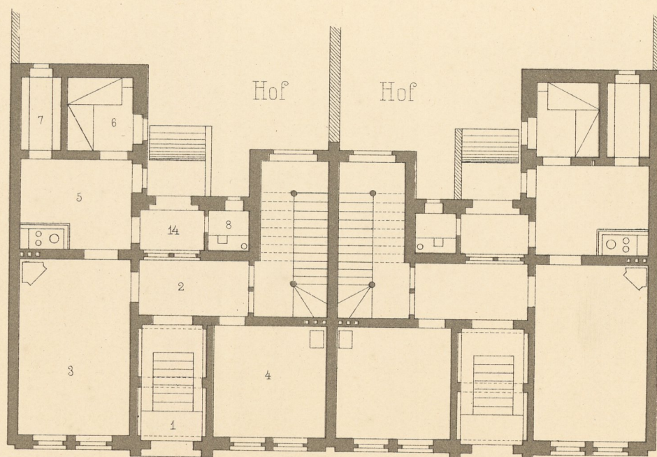
Erdgeschoss.
