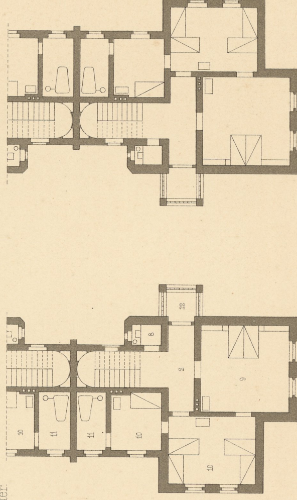
I.er Stock.
