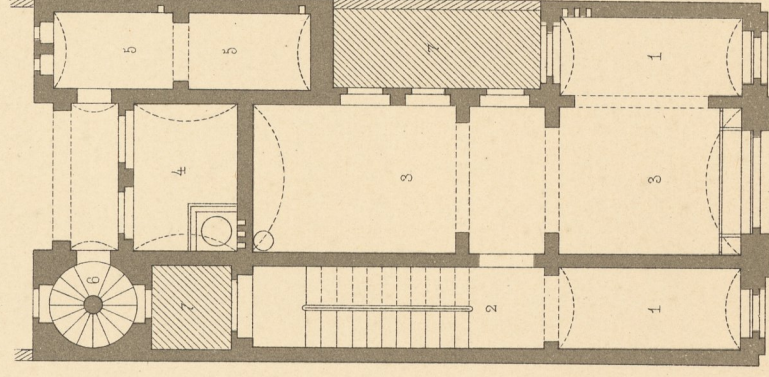
Erdgeſchoſs.
