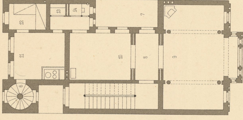
I.ter Stock
