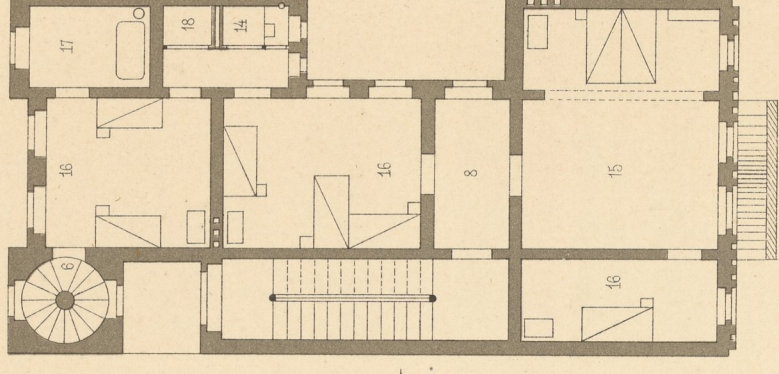
II.ter Stock
