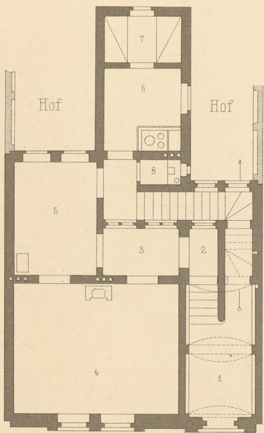
Erdgeschoss.
