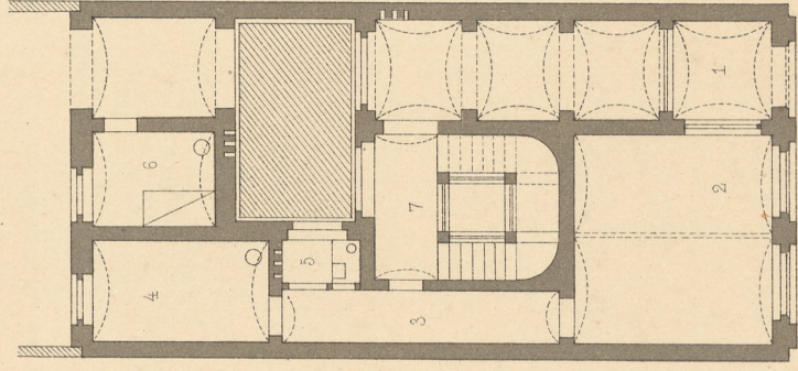
Erdgeschoss.
