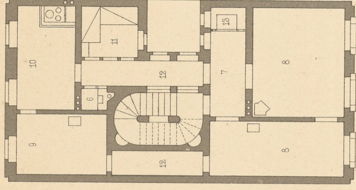
I. Stock.
