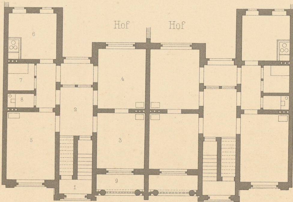
Erdgeschoss.
