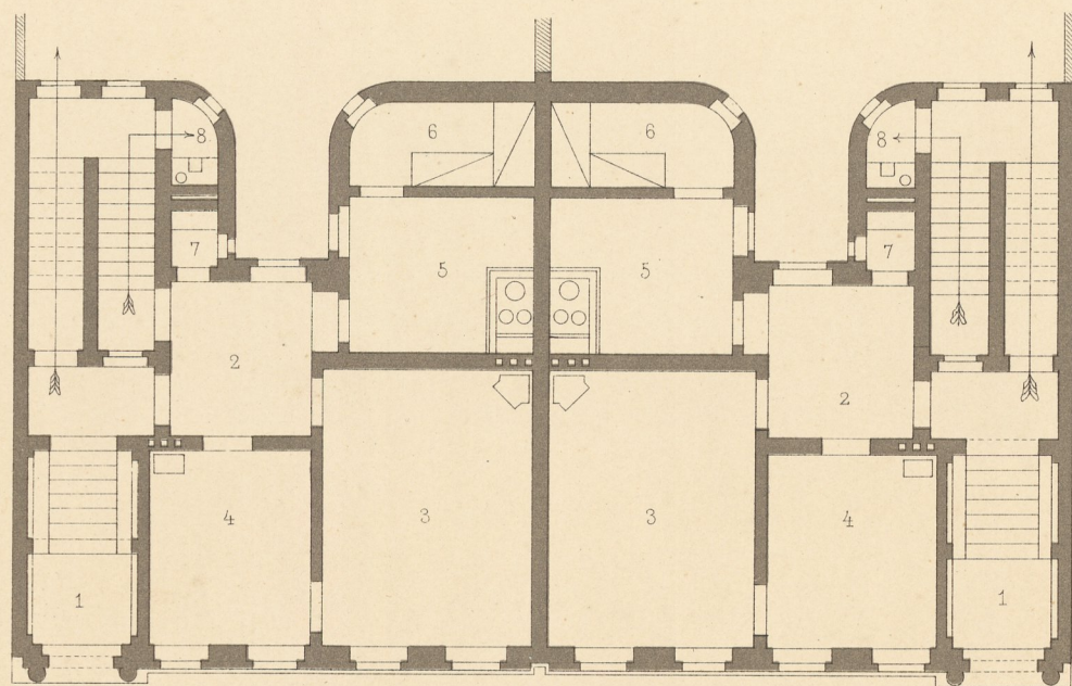
Erdgeschoss.
