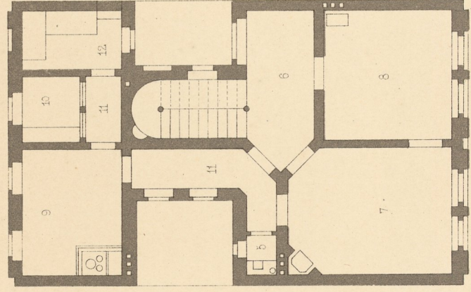
Ier Stock .
