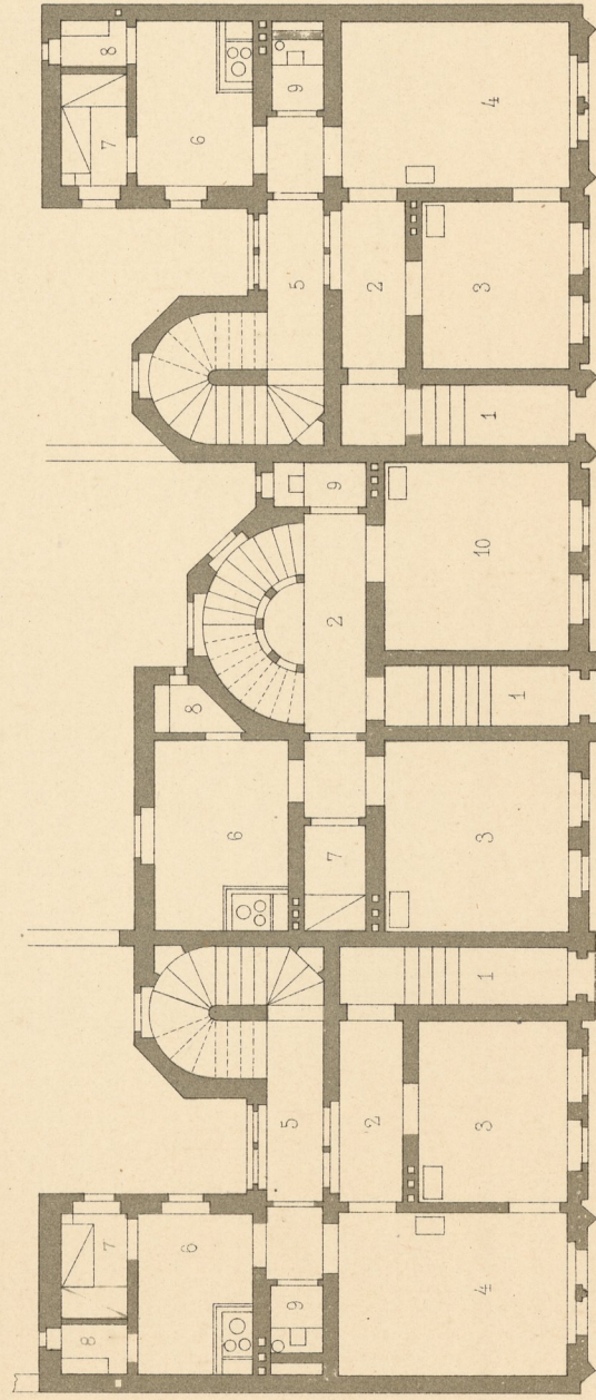
Erdgeschoss.
