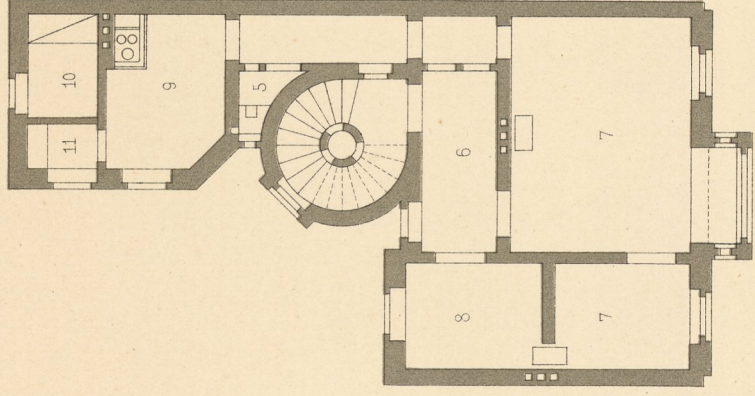
I.ter Stock.
