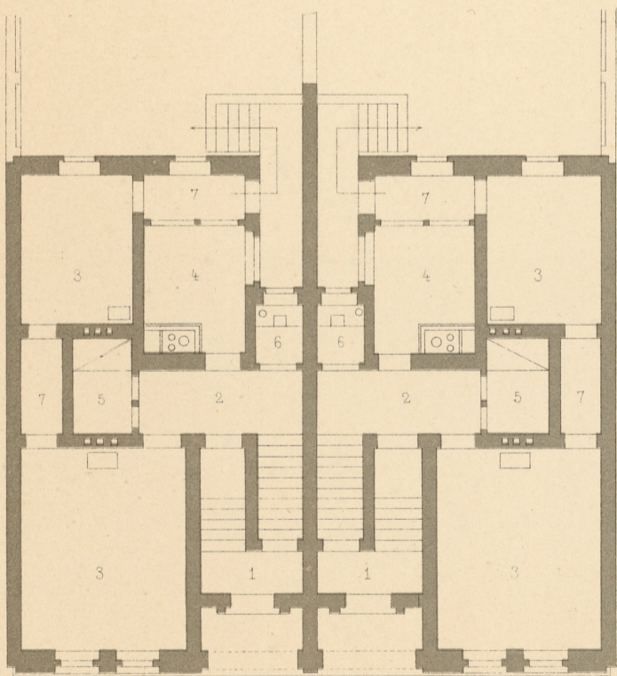
Erdgeschoss.
