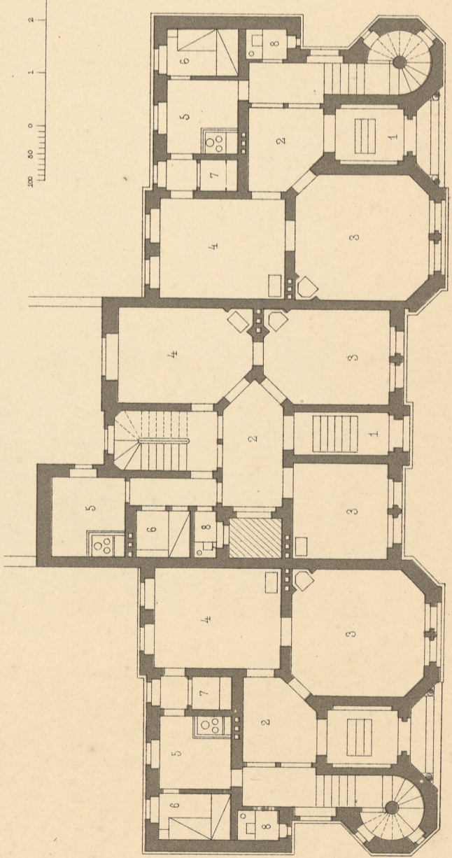
Erdgeschoss.
