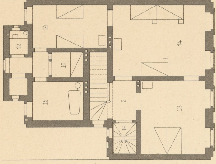
Ier Stock.
