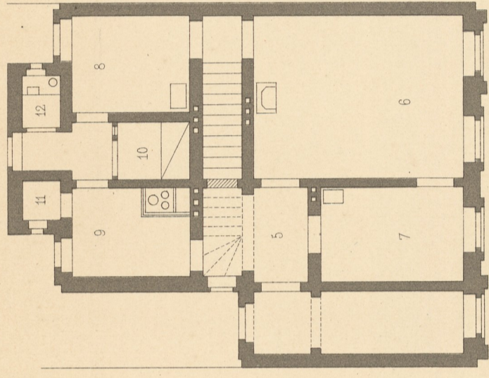
Erdgeschoss.
